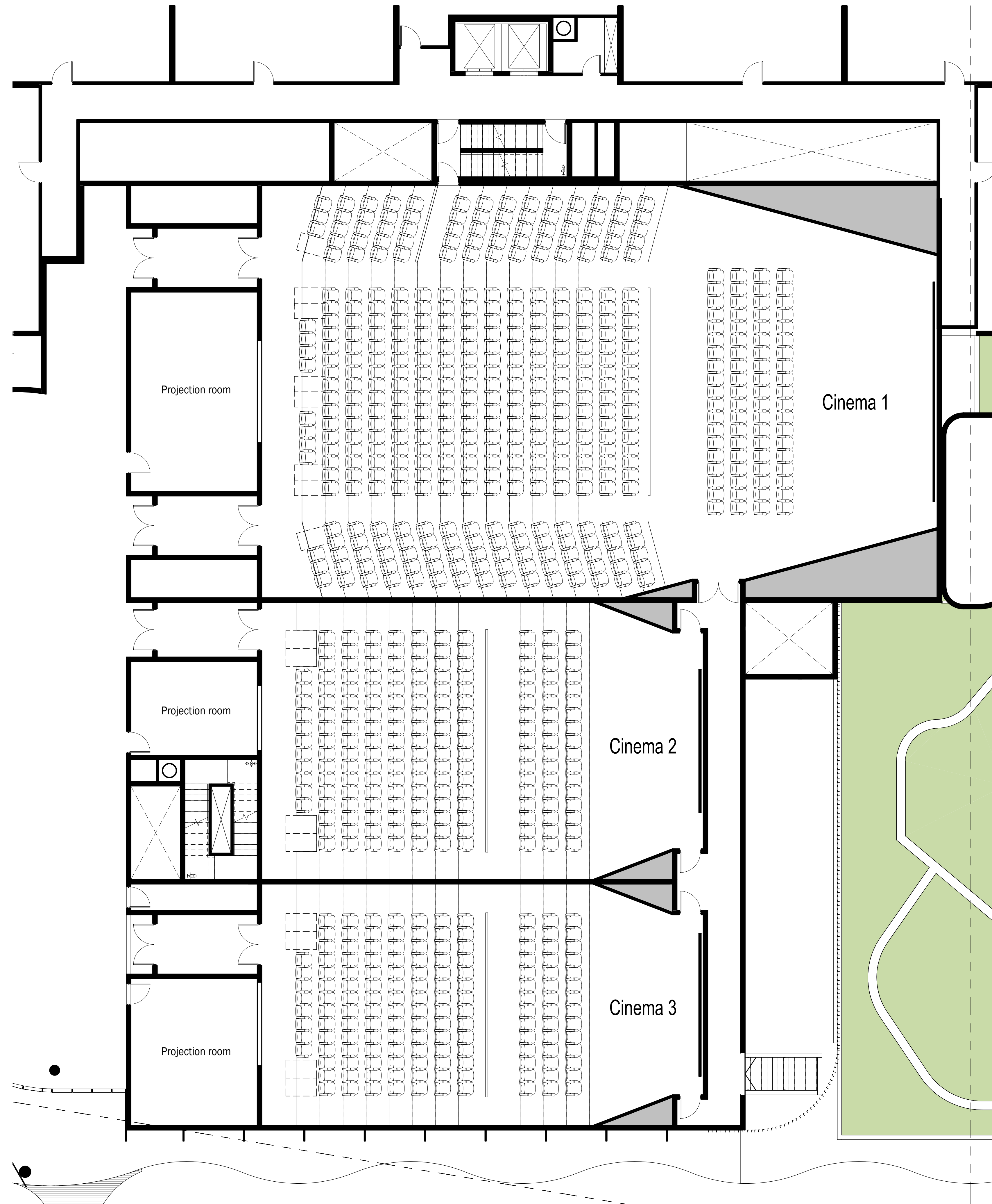
Level 4 - Cinema Plan Scale @ A1 1:100
